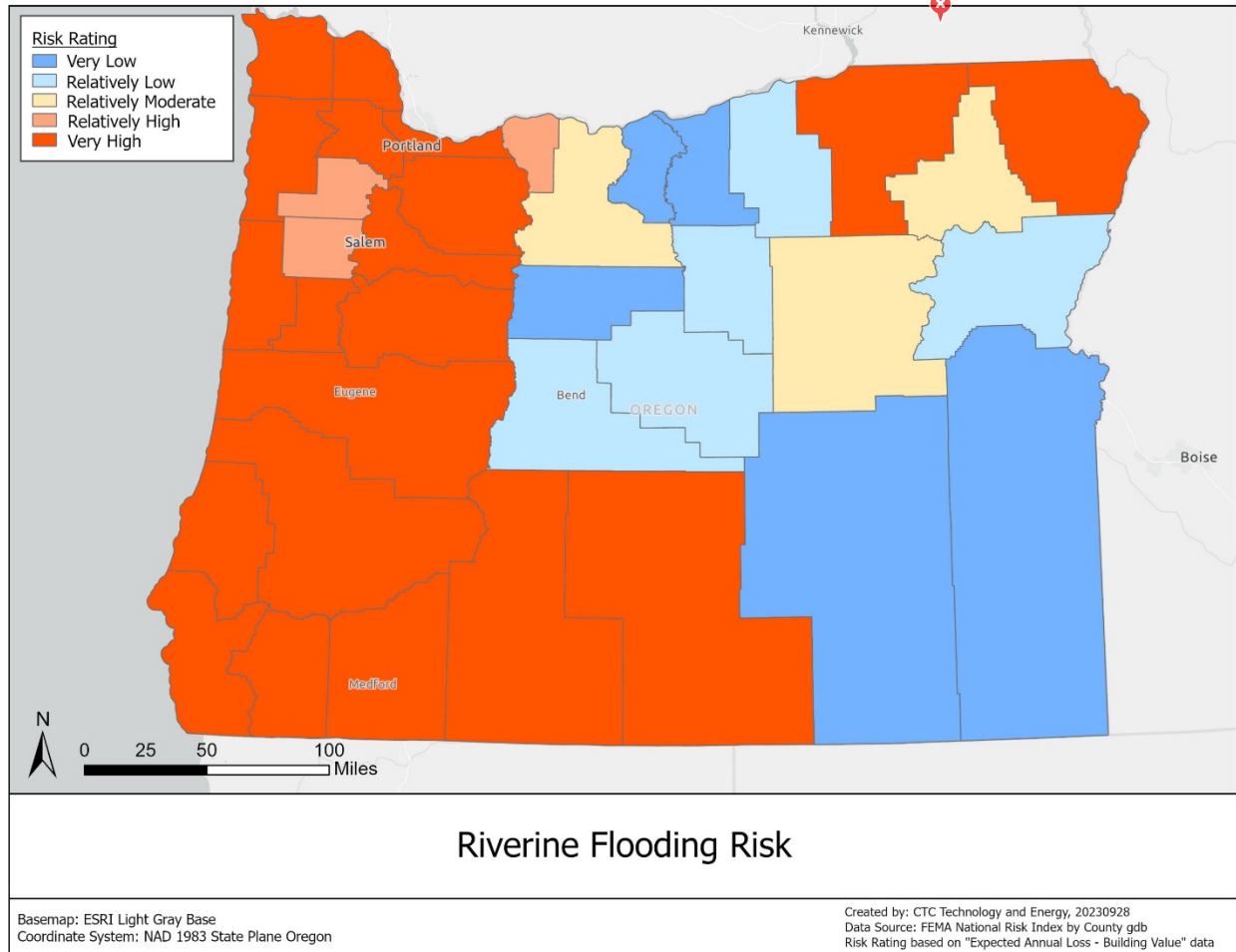
Figure 6: Map of inland flooding risk in Oregon
