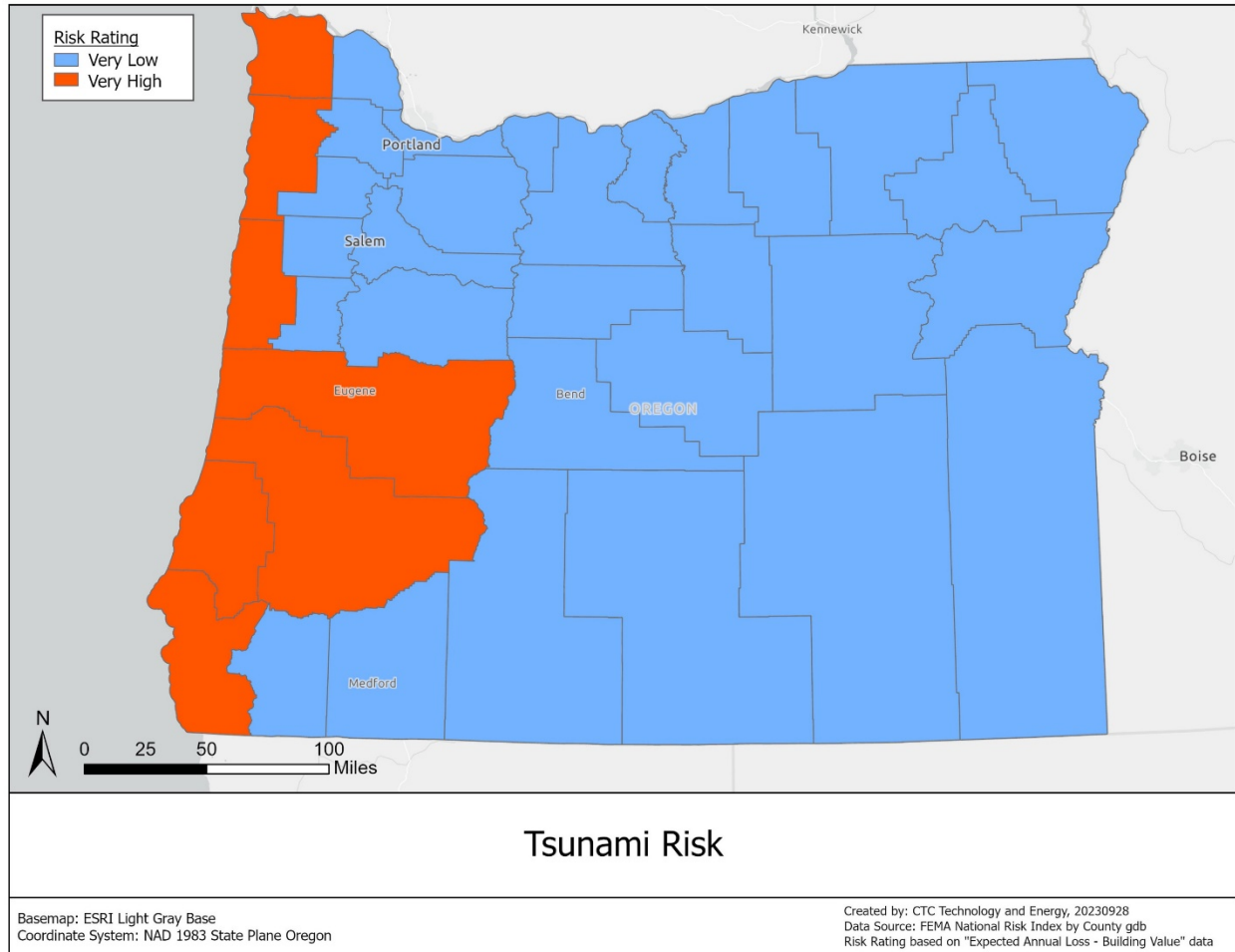
Figure 12: Map of tsunami risk in Oregon
